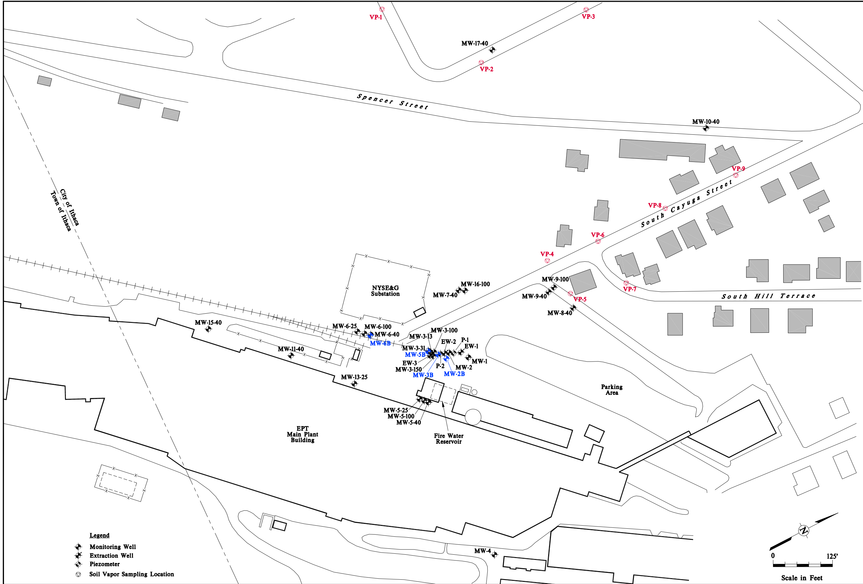
Figure 2 Site Layout and Vadose Zone Sampling Locations Emerson Power Transmission Ithaca, New York
